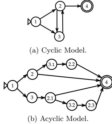
Fig. 2: Unrolling Example.
